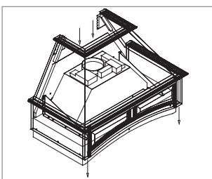
Step 5: Slip the wood range hood on top of the mounting plate
